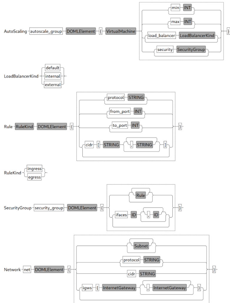
Figure 10. Abstract Infrastructure layer model (part 2/4).
