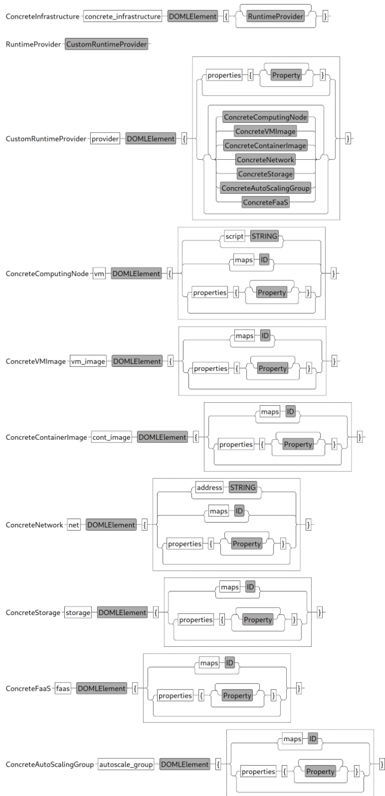
Figure 13. Concrete Infrastructure layer model.
