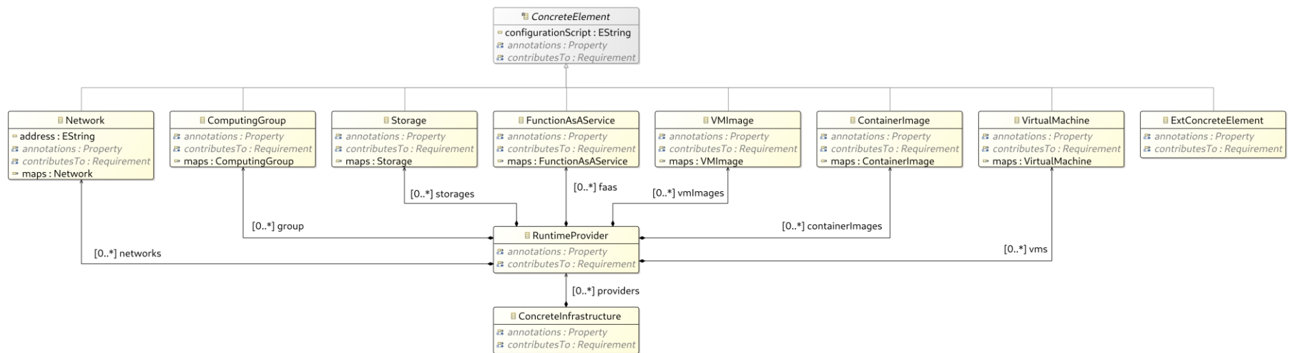
Figure 4. Concrete Infrastructure Layer diagram
