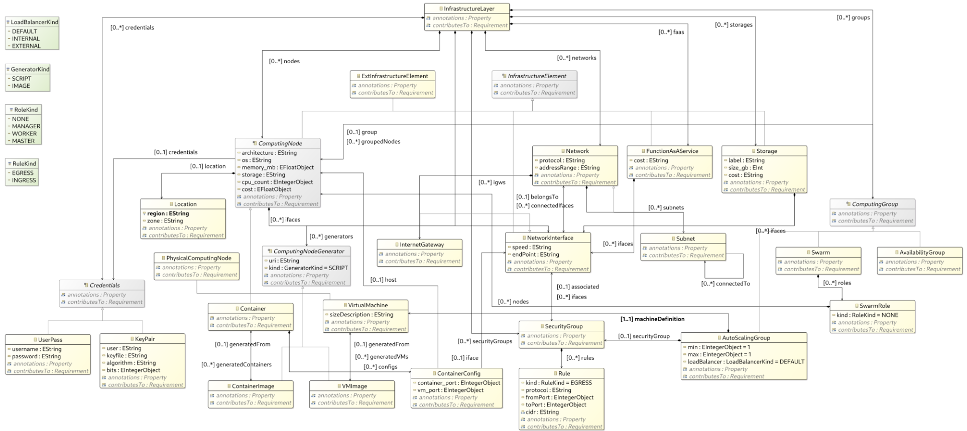
Figure 3. Infrastructure layer diagram
