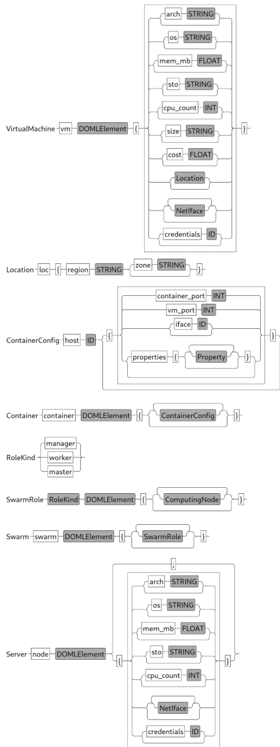
Figure 12. Abstract Infrastructure layer model (part 4/4).
